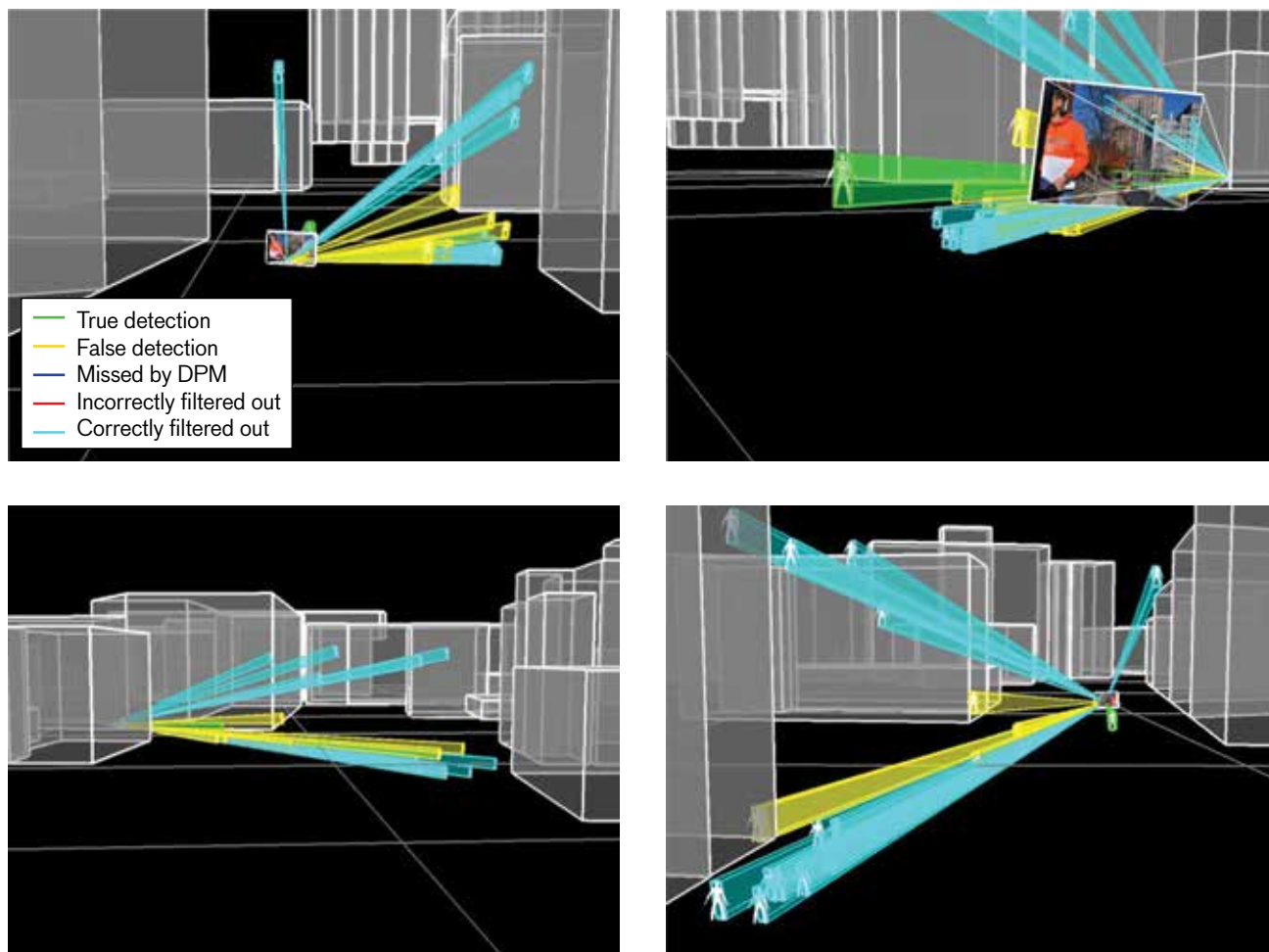
FIGURE 23. Figure 22's detection results after the false-alarm filters are applied are shown in 3D space, with four different views depicted.
