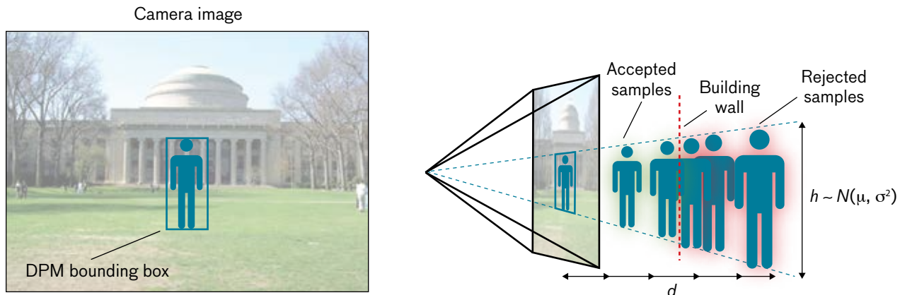
FIGURE 25. A sample-based approach allows for the relaxation of the height assumption; \mu is the average height of a person and \sigma is the standard deviation.
