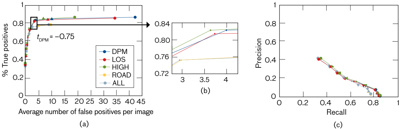
FIGURE 28. ROC (a) and precision-recall (c) curves are shown for car detection using a deterministic 1.5-meter height estimate. A zoomed-in ROC curve is shown in (b).
