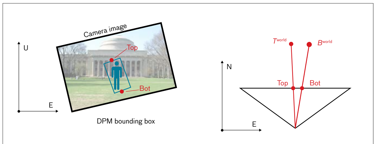
FIGURE 19. The figure illustrates the effect of the camera's y -axis not being parallel to the world u -axis.
